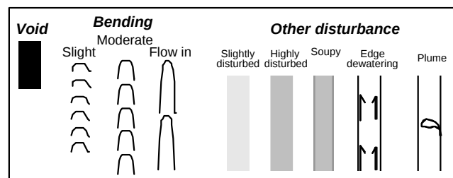
Fig. 5.6d. Coring disturbance
